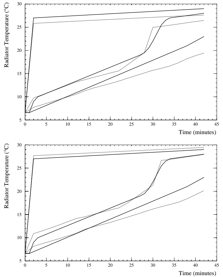
Figure 5: Pre- and Post-correlation Predictions of a CPL Condenser/Radiator Transient Event
