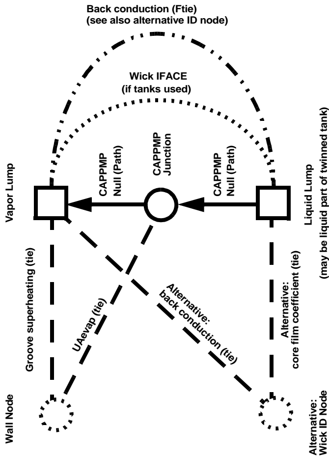
Figure 3: Two Possible Models of a Section of Primary Wick
