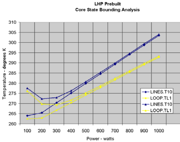
Figure 7: Core Bounding Analysis
